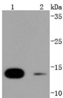
Fig. 1. Western blot analysis of SUMO4 on different lysates using anti-SUMO4 antibody at 1/1,000 dilution. Positive control: Lane 1: 293T; Lane 2: Jurkat
